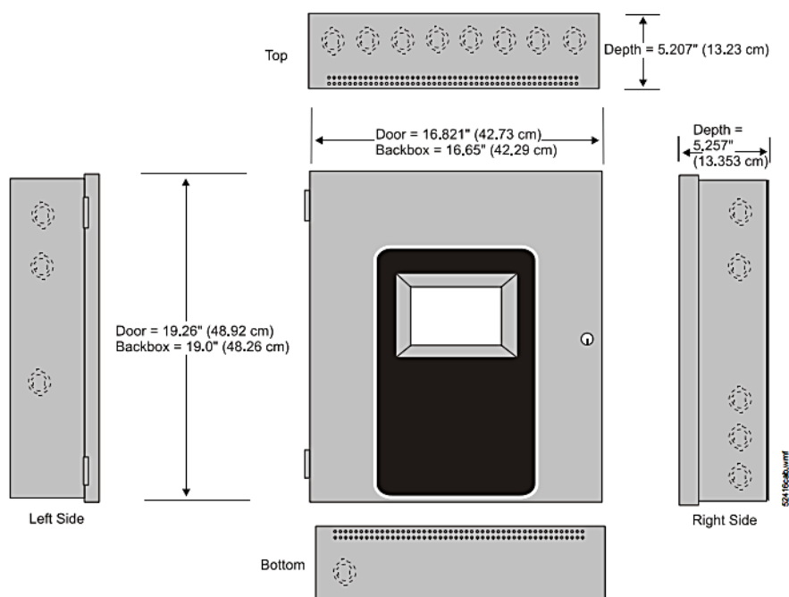
Cabinet Measurements
