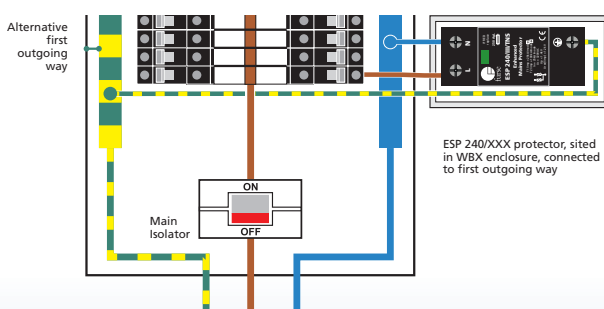
Figure 2: ESP 240/XXX Protector connected to the nearest available outgoing (MCB) way to the incoming supply. Since there is insufficient space within the distribution board the ESP Protector has been mounted within a separate enclosure, directly alongside the board.
